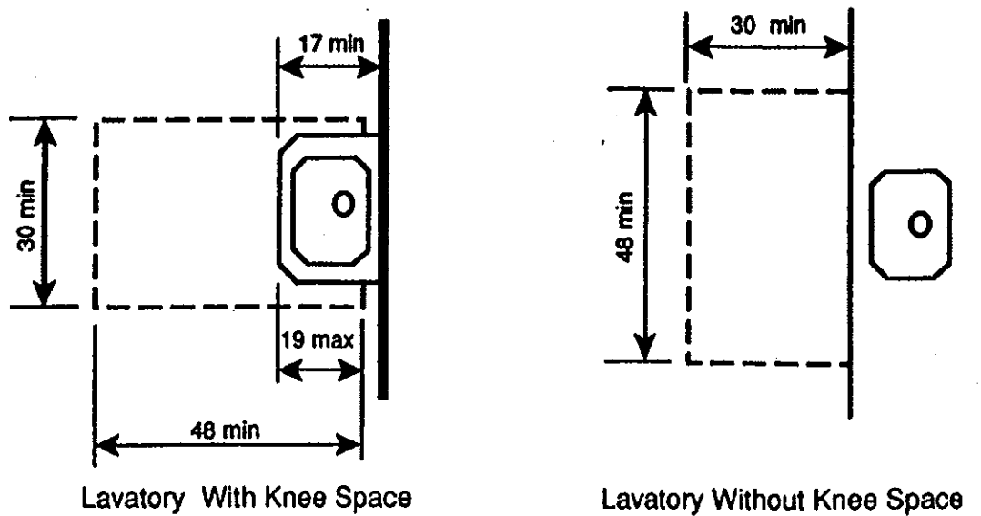
Clear Floor Space at Lavatories
