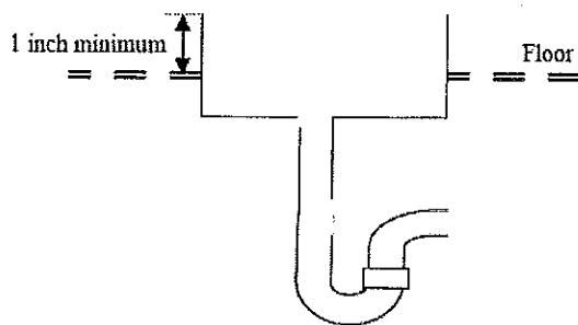
WASTE SINK IN FLOOR
