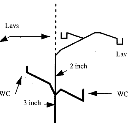
Common vents serving as a wet vent
