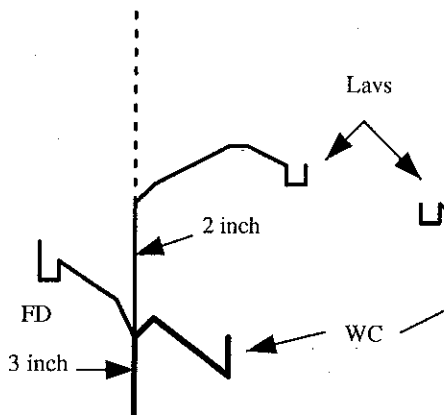
Individual vent serving as a wet vent
