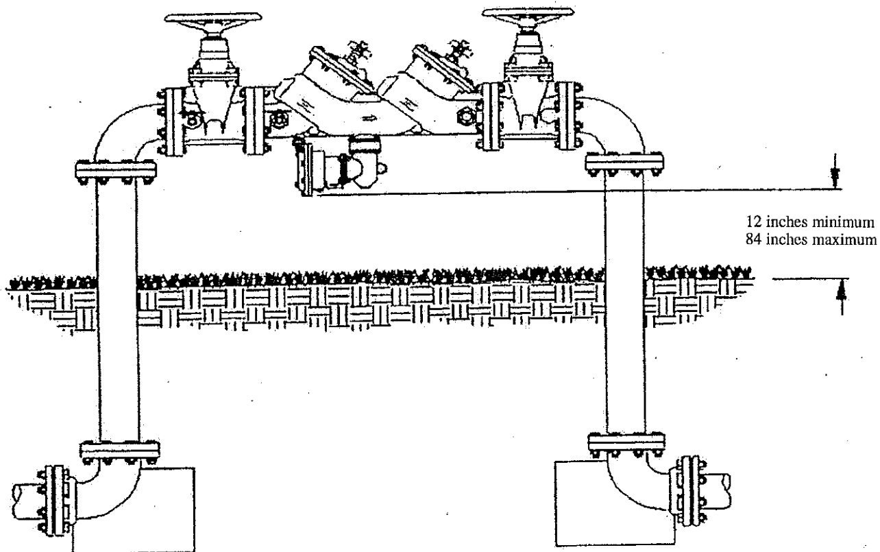
REDUCED PRESSURE ASSEMBLY OUTDOOR INSTALLATION
