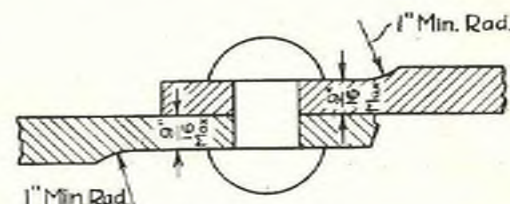
Fig. 1. Circumferential Joint for Thick Plates of Horizontal-Return Tubular Boilers.
