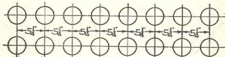
Fig. A-8. Example of Tube Spacing with Pitch of Holes Equal in Every Row.
