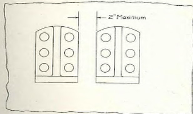
Fig. 14. Spacing of Supporting Lugs in Pairs on H. R. T. Boilers.
