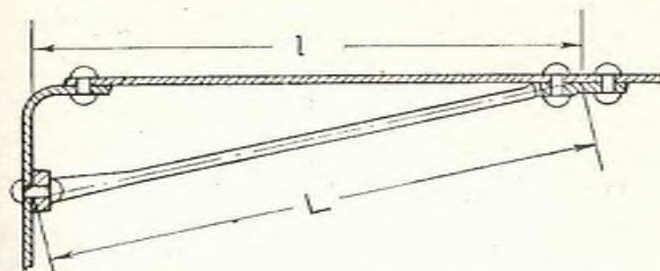
Fig. 7. Measurements for determining stresses in diagonal stays.
