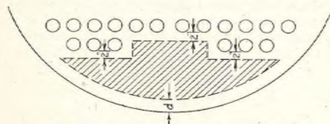
Fig. 6. Method of Determining Net Area of Irregular Segment of a Head.
