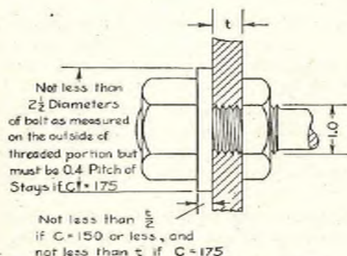
Fig. 3. Acceptable proportions for Ends of Through Stays.
