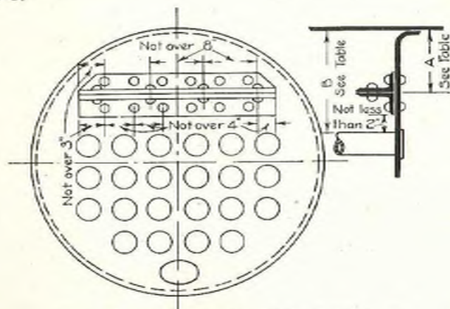
Fig. 8. Staying of Head with Steel Angles in Tubular Boiler.
