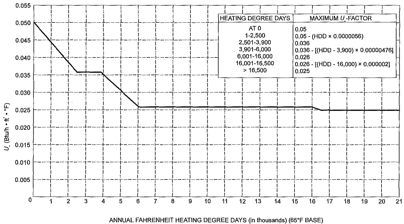
FIGURE 502.2(2) U_o -FACTORS—ROOF/CEILINGS
