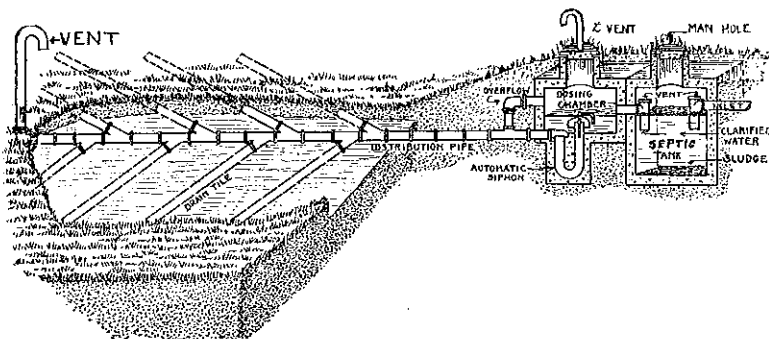
(45) Illustrating sewage, disposal system consisting of septic tank, dosing chamber, siphon and drainage tile. H 62.20 (2) (c), (8).
