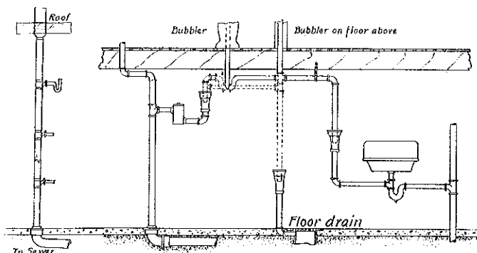
(35) Illustrating four approved methods of connecting drinking fountain wastes. H 62.07 (3), H 62.14 (5).
