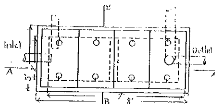
Plan of Grease Basin
