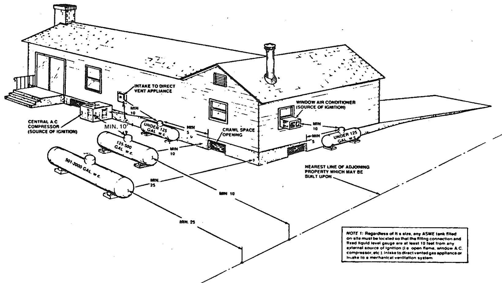
Figure G-2 Aboveground ASME Tanks (This figure for illustrative purposes only; text shall govern.)
