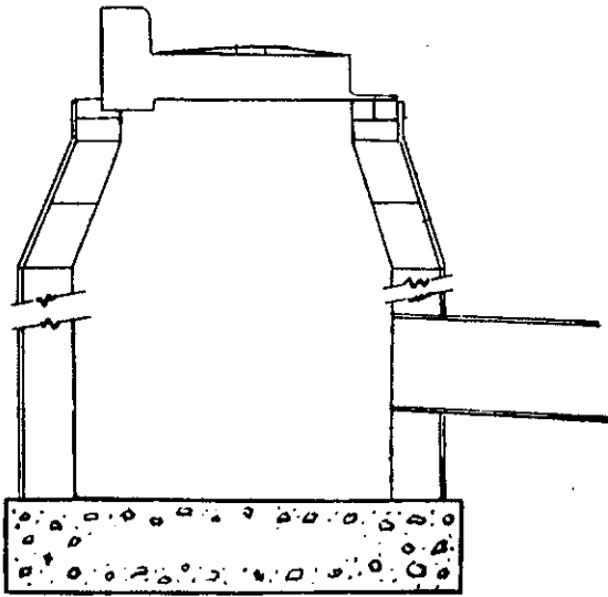
STANDARD STORM WATER CATCH BASIN (MASONRY)
