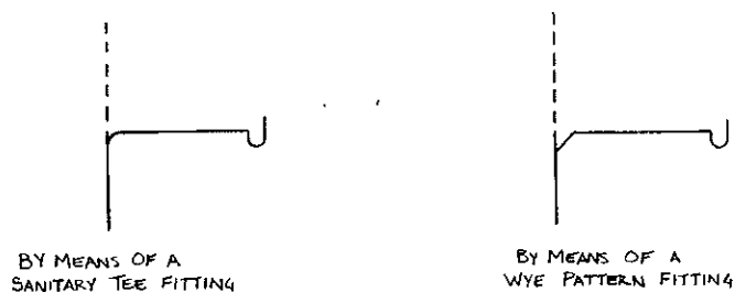
VENT CONNECTING TO VERTICAL DRAIN PIPING
