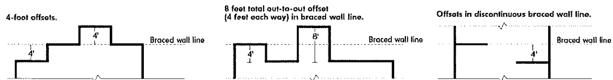
FIGURE 21.25-C PERMITTED OFFSETS
