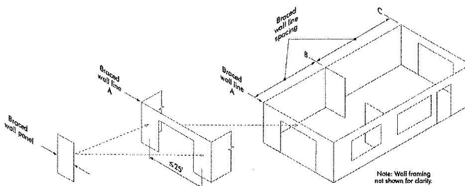
FIGURE 21.25-A BRACED WALL PANELS AND BRACED WALL LINES
